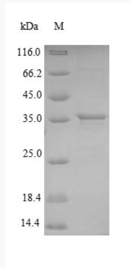
(Tris-Glycine gel) Discontinuous SDS-PAGE (reduced) with 5% enrichment gel and
