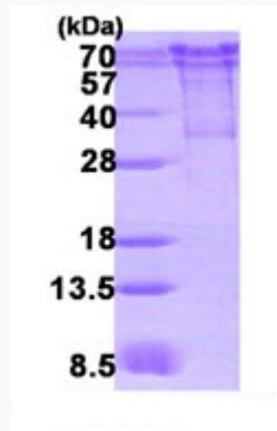
15% SDS-PAGE (3ug)
