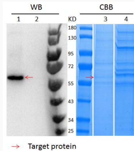
SDS-PAGE analysis of purified human cxcr4, 5 ul/Line.
