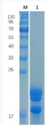
Reducing 12% SDS-PAGE analysis profile of purified Cynomolgus IL1RN (CBB stained).
