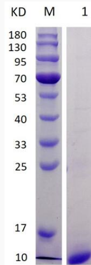
12% SDS-PAGE analysis profiles of purified ProInsulin-47AC (CBB stained).
