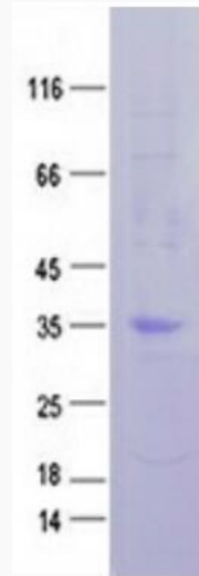
Coomassie blue staining of purified MYADM protein.
