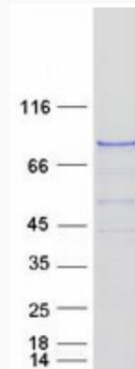
Coomassie blue staining of purified OSBPL10 protein.
