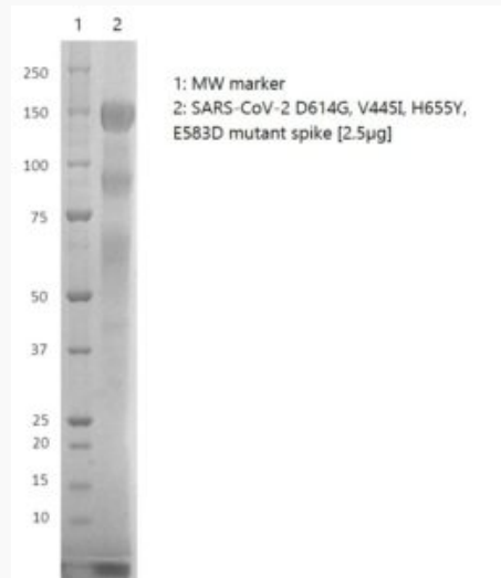
Coomassie-stained SDS-PAGE showing purified D614G, V445I, H655Y, E583D mutant Spike protein.
