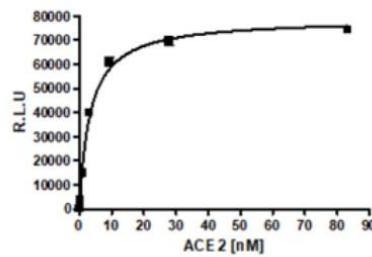
SARS-CoV-2 Spike Trimer (S1+S2): ACE2 Binding
