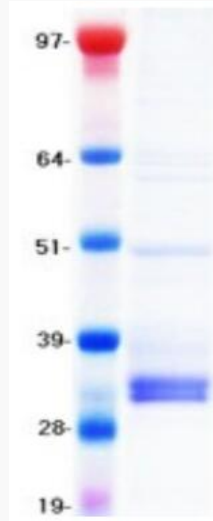
Coomassie blue staining of purified TIGIT protein.
