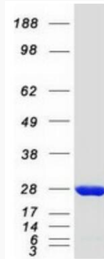
Coomassie blue staining of purified UCHL3 protein.
