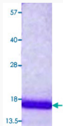
15% SDS-PAGE Stained with Coomassie Blue
