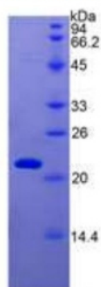
Human IL17RA
