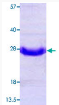
15% SDS-PAGE Stained with Coomassie Blue
