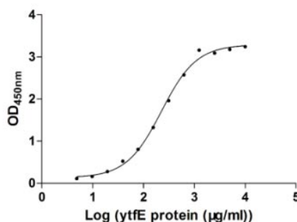
The Binding Activity of aqpZ with ytfE
