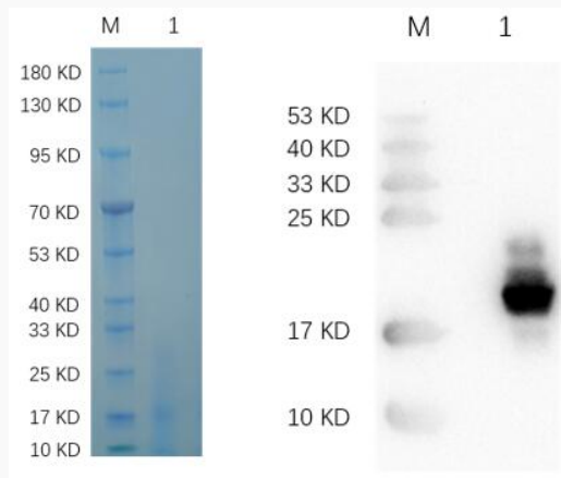
Reducing 12% SDS-PAGE and WB analysis profile
