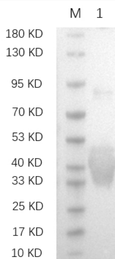
Reducing 12% SDS-PAGE and WB analysis profiles of purified LEFTY1
