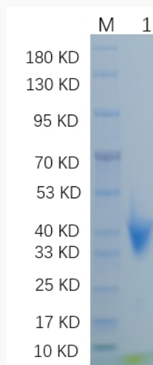
Reducing 12% SDS-PAGE and WB analysis profiles of purified LEFTY1
