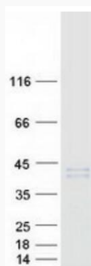
Coomassie blue staining of purified HSD11B1 protein.
