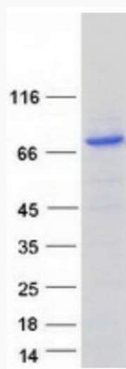
Coomassie blue staining of purified SARM1 protein.
