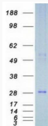
Coomassie blue staining of purified DIRAS3 protein.
