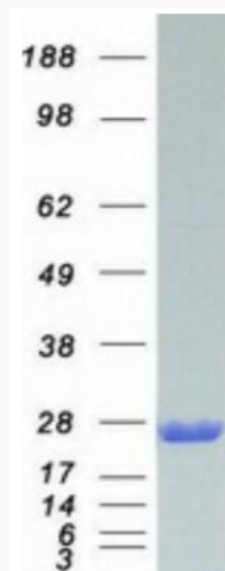
Coomassie blue staining of purified TAGLN2 protein.
