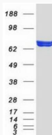
Coomassie blue staining of purified DARS2 protein.
