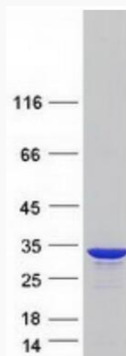
Coomassie blue staining of purified HSD17B14 protein.
