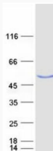
Coomassie blue staining of purified USP3 protein.
