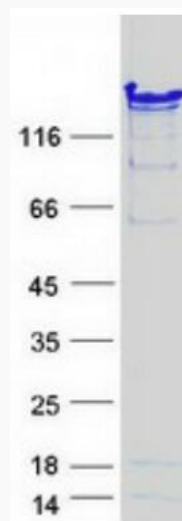
Coomassie blue staining of purified NASP protein.
