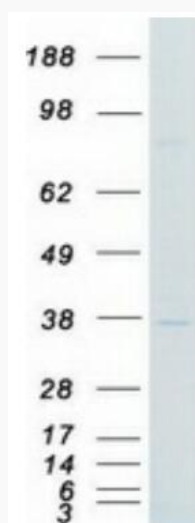
Coomassie blue staining of purified CDK1 protein.
