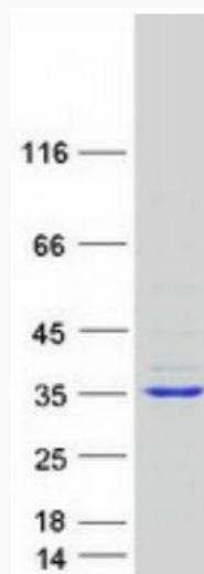
Coomassie blue staining of purified TTC33 protein.
