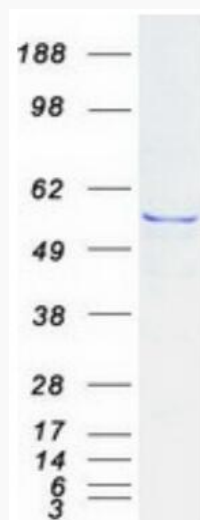
Coomassie blue staining of purified IFIT1 protein.
