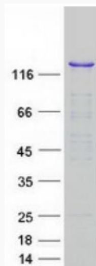
Coomassie blue staining of purified SF3B2 protein.
