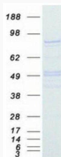
Coomassie blue staining of purified SUZ12 protein.
