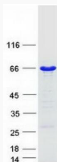
Coomassie blue staining of purified G3BP1 protein.
