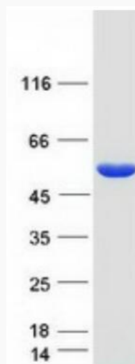
Coomassie blue staining of purified GSDMA protein.
