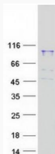
Coomassie blue staining of purified MACC1 protein.
