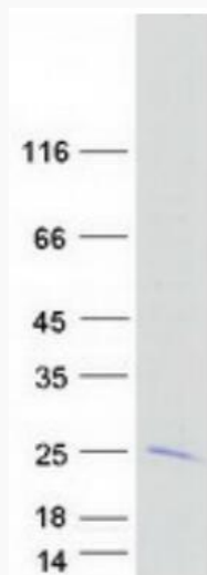
Coomassie blue staining of purified TMEM240 protein.
