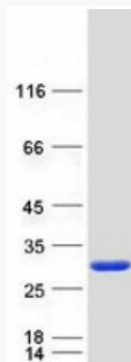
Coomassie blue staining of purified STYX protein.
