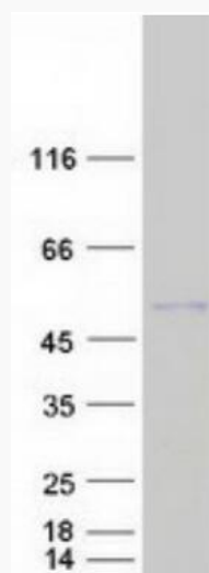
Coomassie blue staining of purified AMBP protein.
