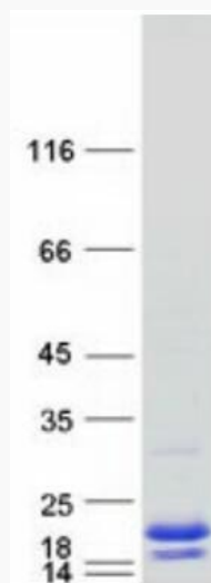
Coomassie blue staining of purified TSC22D3 protein.
