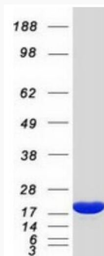
Coomassie blue staining of purified NME1 protein.
