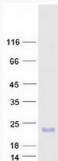
Coomassie blue staining of purified MLANA protein.
