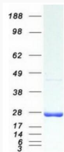
Coomassie blue staining of purified RAB1A protein.
