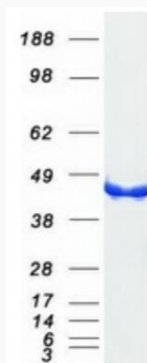
Coomassie blue staining of purified CKB protein.
