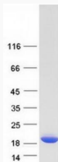
Coomassie blue staining of purified TTR protein.
