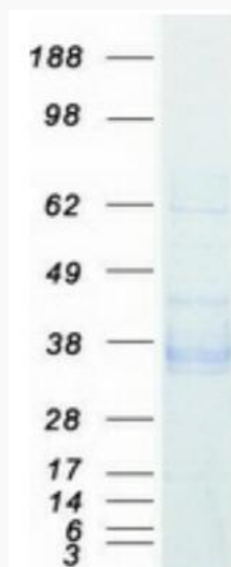
Coomassie blue staining of purified EPCAM protein.
