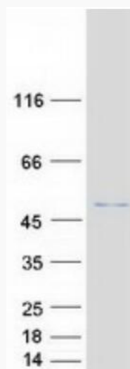
Coomassie blue staining of purified SPDEF protein.
