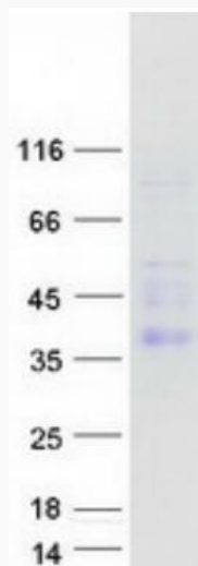
Coomassie blue staining of purified CEACAM4 protein.
