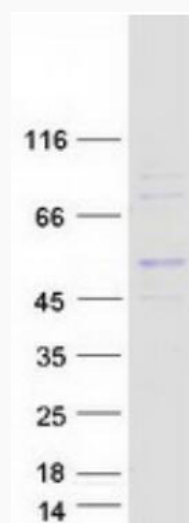
Coomassie blue staining of purified MRPS30 protein.
