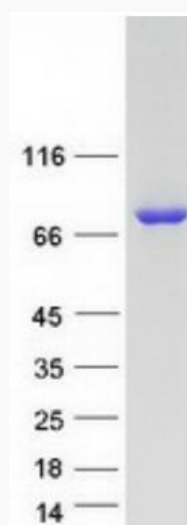
Coomassie blue staining of purified SHKBP1 protein.
