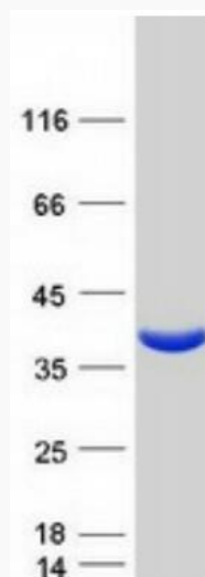
Coomassie blue staining of purified CASTOR1 protein.
