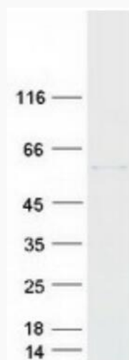
Coomassie blue staining of purified CYP2W1 protein.
