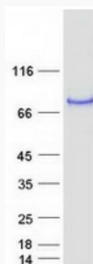
Coomassie blue staining of purified CAPN13 protein.
